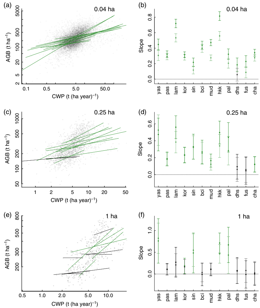
Fig. 4. Panels a, c, e: observed relationships between coarse woody productivity (CWP) and above-ground biomass (AGB) at the study sites at three spatial grains (0.04 ha, 0.25 ha, 1 ha). Points show individual quadrat data, and lines show fitted models (green = statistically significantly positive). Axis scales are logarithmic. Panels b, d, f: strengths of relationships with closed circles showing slopes from panels a, c, e, and solid whiskers showing 95% confidence intervals, and open circles with dashed whiskers showing slopes and confidence intervals from the analysis controlling for stem density. Site name abbreviations on horizontal axes are given in Table 1.
